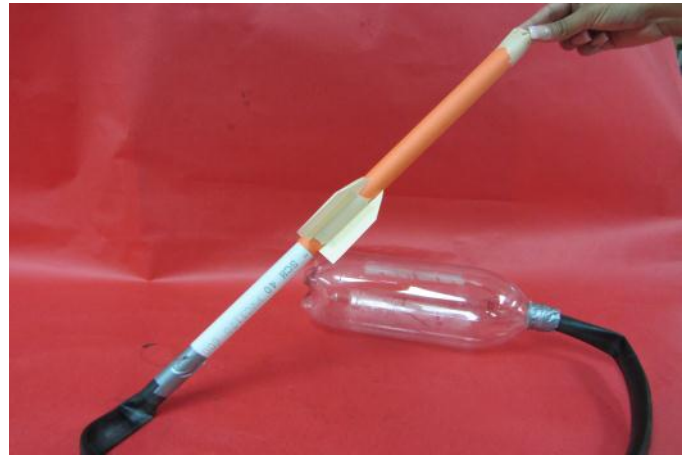
Slide the rocket onto the free end of PVC pipe, stomp on the 2-liter bottle and watch the rocket launch!
